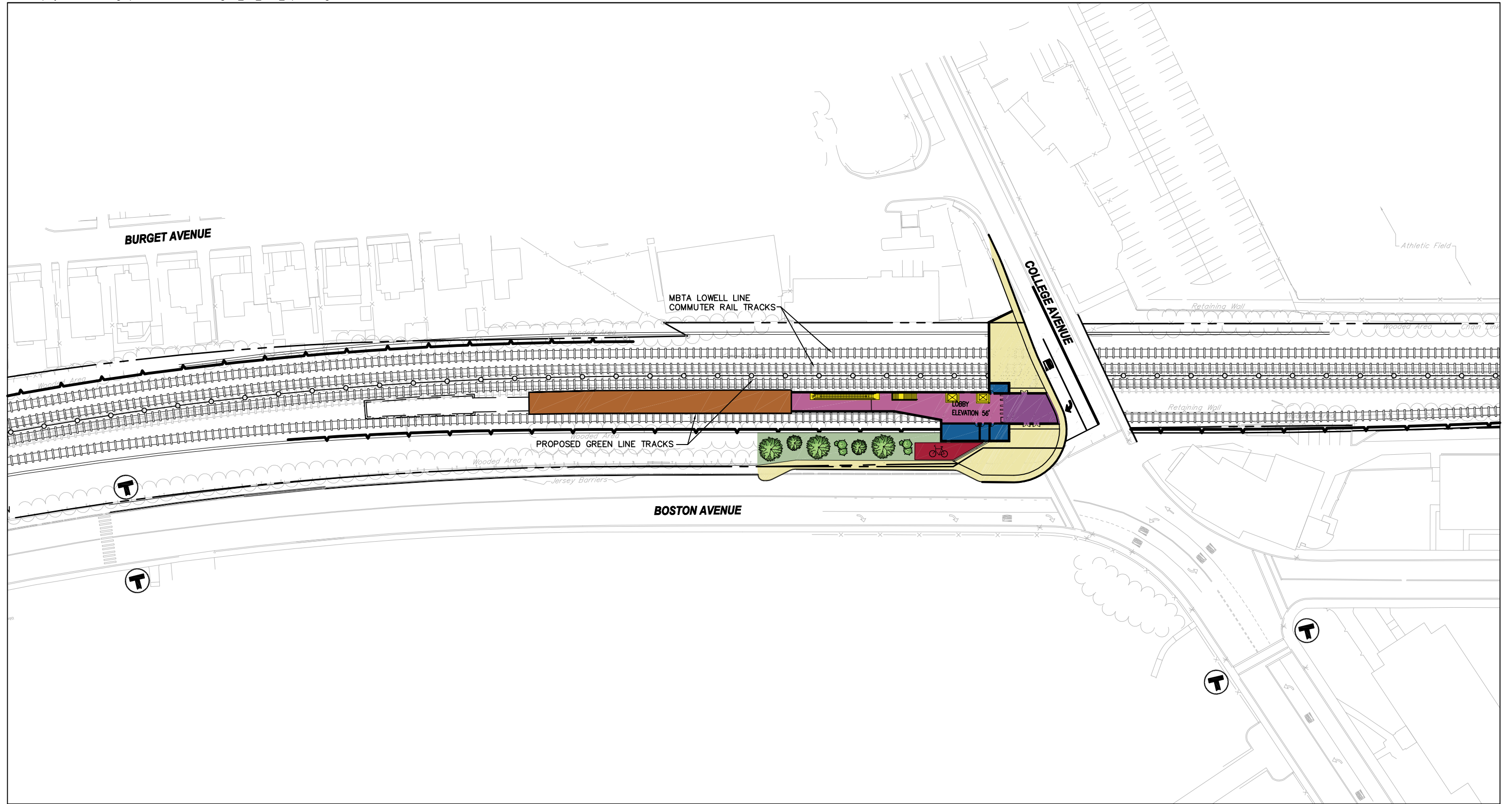
Figure 3.7-23 College Avenue Station Alternatives 2, 4, 5 Station Layout
