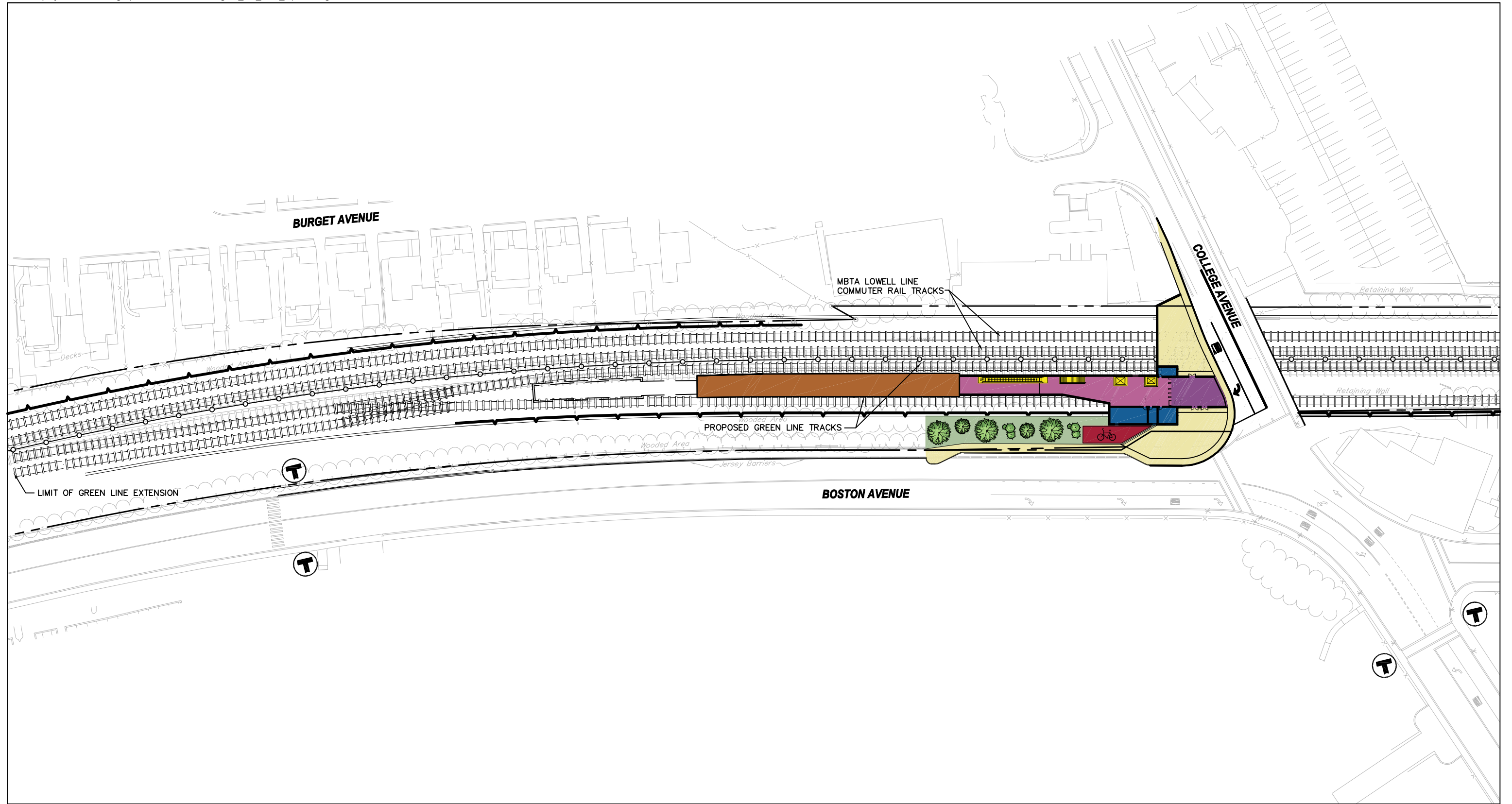
Figure 3.7-22 College Avenue Station Medford Hillside Terminus Alternatives 1, 3 Station Layout
