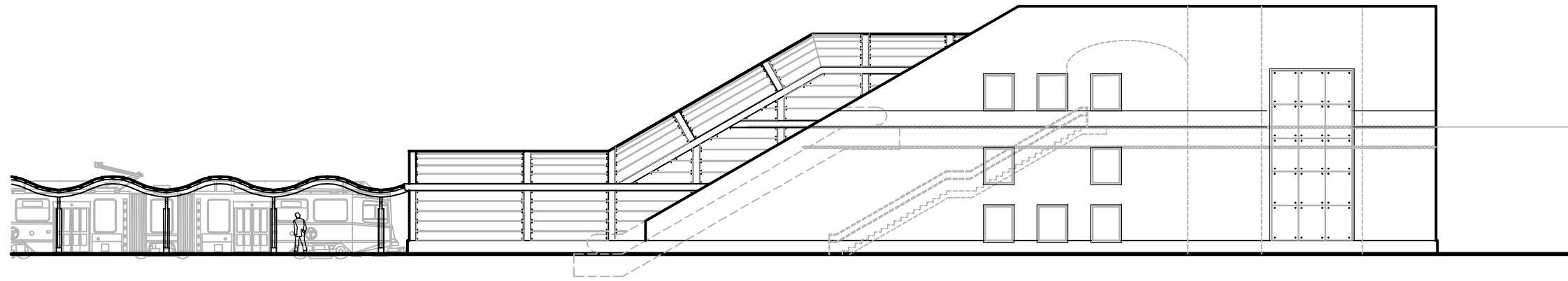
SOUTH ELEVATION
