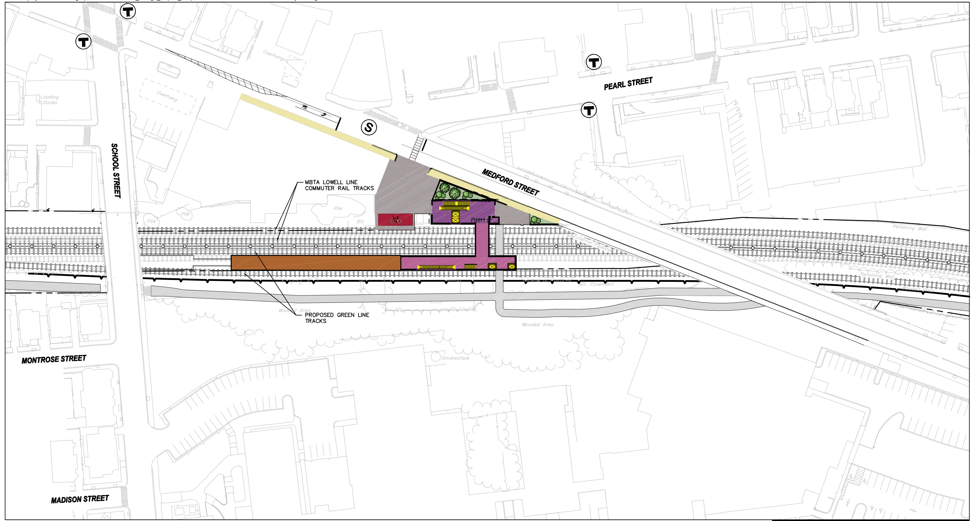
Figure 3.7-10 Gilman Square Station Station Layout
