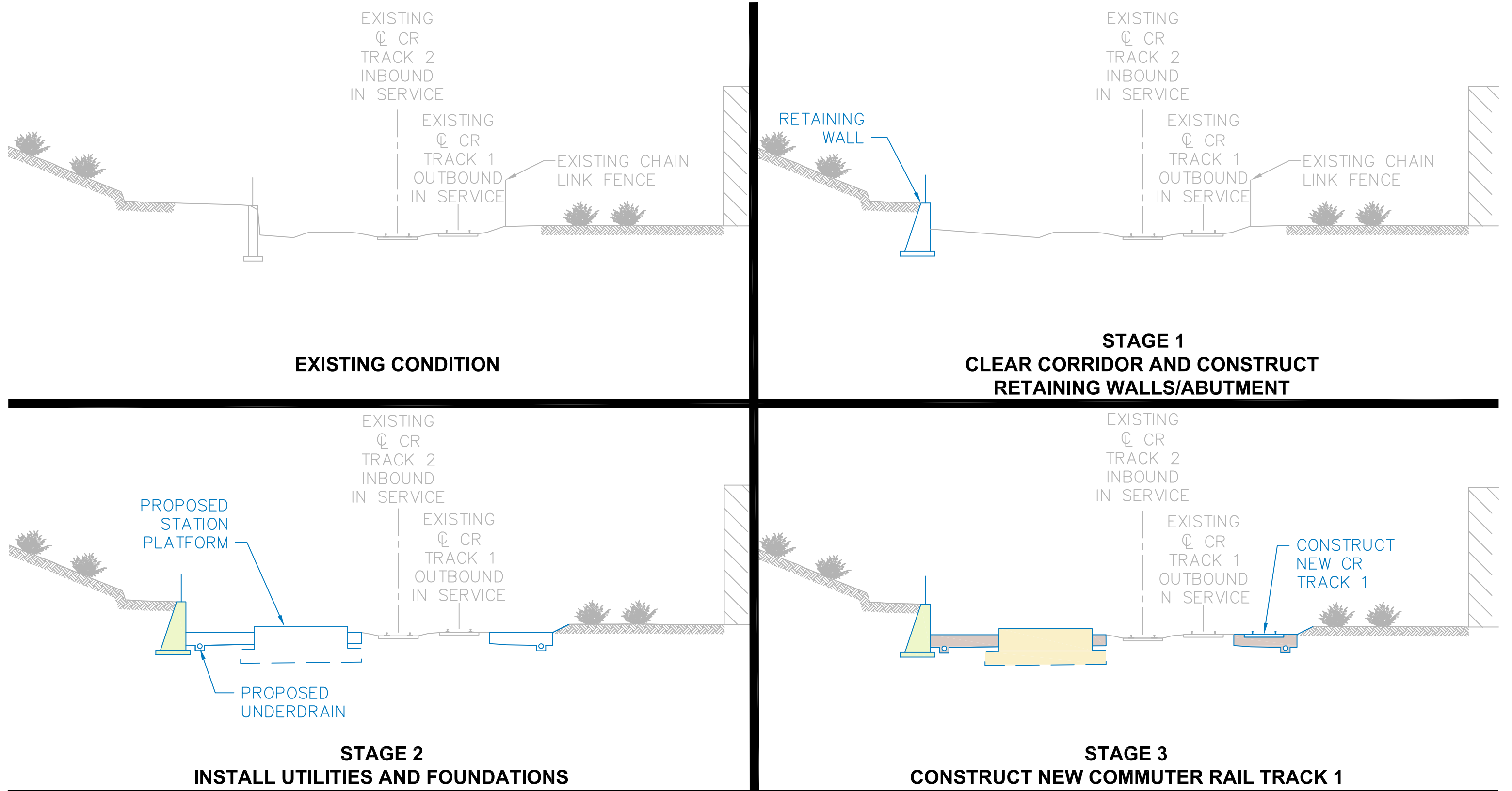
Figure 8-5 Typical Construction Staging Sheet 1 of 2
